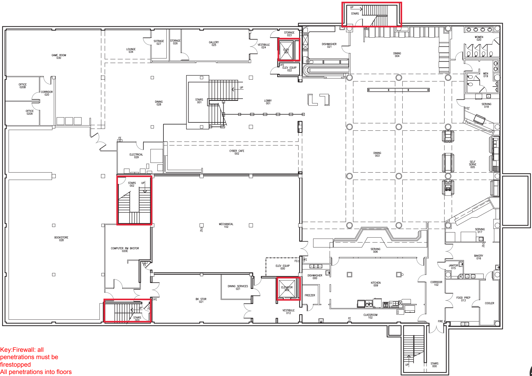
1 STUDENT CENTER BUILDING BASEMENT FLOOR PLAN SCALE: 1/16" = 1'-0"
