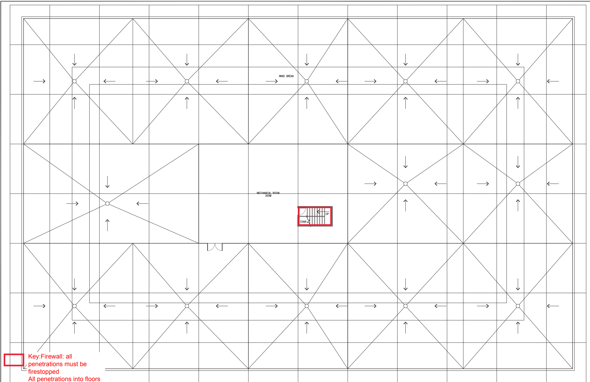
1 STUDENT CENTER BUILDING ROOF PLAN SCALE: 1/16" = 1'-0"
