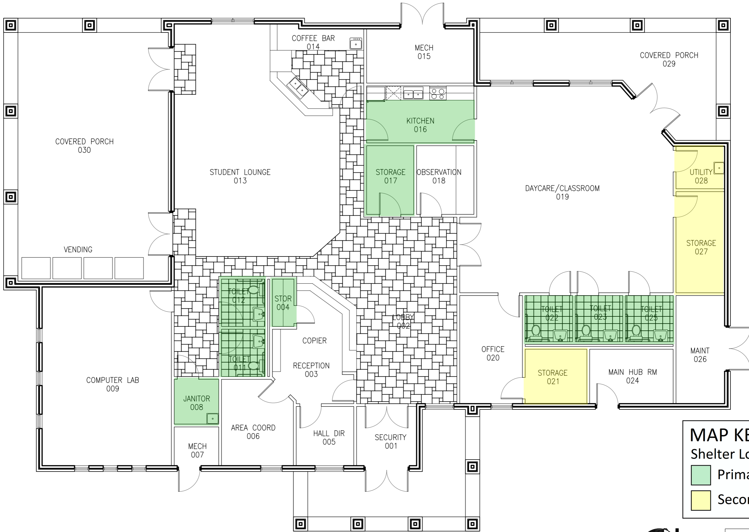
1 LOWERY WOODS CLUB HOUSE 1ST FLOOR PLAN SCALE: 1/8" = 1'-0"
