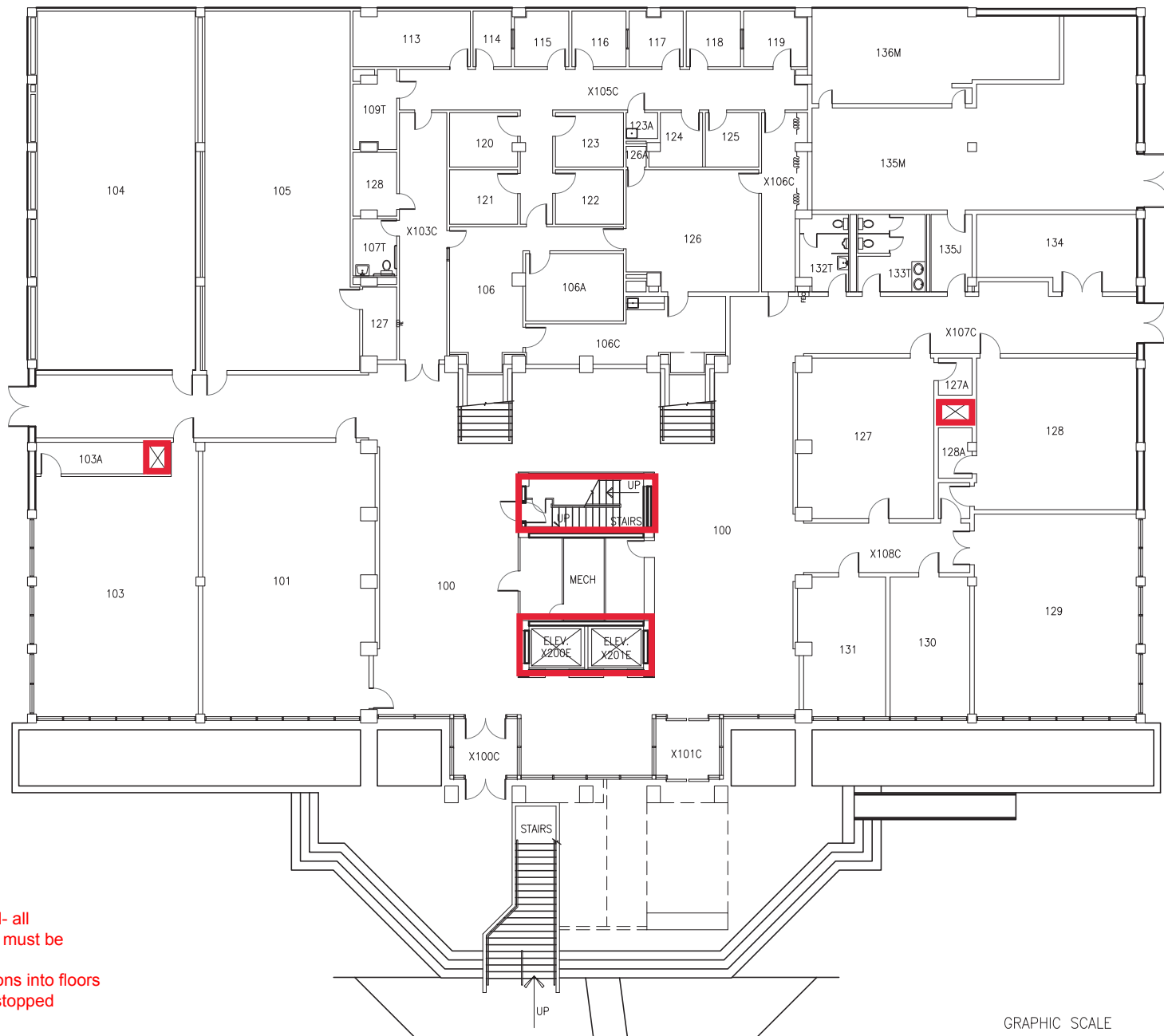
1 CLASSROOM FACULTY OFFICES BUILDING 1ST FLOOR PLAN
